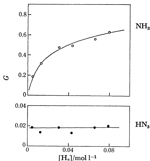
Fig. 1. G -Values of ammonia ( \circ ) and hydrogen azide ( \bullet ) as functions of the concentration of hydrogen from the liquid nitrogen solution.
