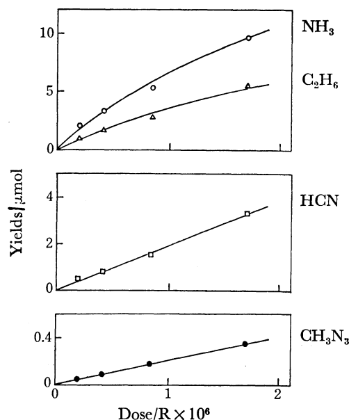
Fig. 2. The dose dependence of the yields of ammonia ( \circ ), ethane ( \Delta ), hydrogen cyanide ( \square ), and methyl azide ( \bullet ) from the \gamma -radiolysis of a liquid nitrogen solution of 0.03 \text{ mol l}^{-1} methane.
