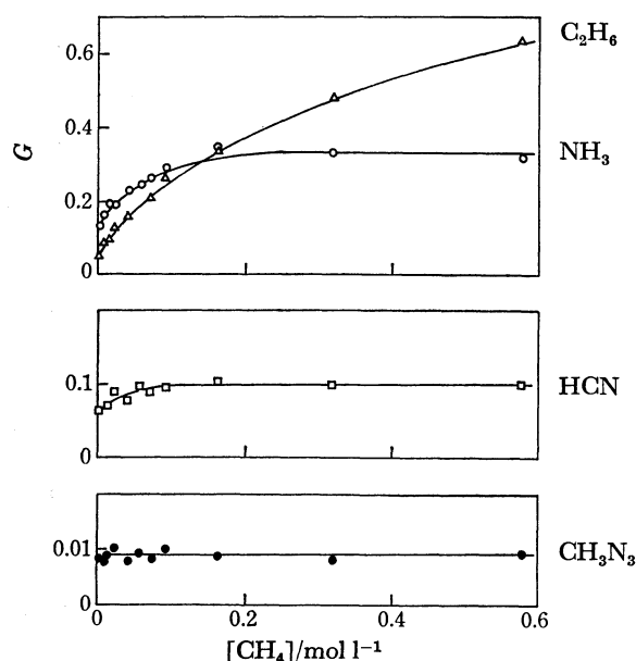
Fig. 3. G -Values of ammonia ( \circ ), ethane ( \Delta ), hydrogen cyanide ( \square ), and methyl azide ( \bullet ) as functions of the concentration of methane from the liquid nitrogen solution.
